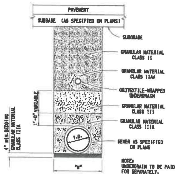
SEWER WITH UNDERDRAIN UNDER ROADBED PLASTIC PIPE
